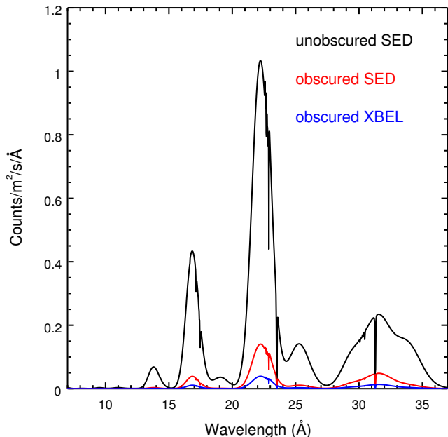
Fig. 8. Photoionization calculations of the X-ray broad emission lines (XBEL). In all three cases below, line profiles are corrected for the redshift and Galactic absorption of NGC 3783. The black solid curve corresponds to a case where the XBEL is directly exposed to the intrinsic SED of 11 December 2016. The red curve is for a case where the XBEL is exposed to the obscured SED of 11 December 2016. The blue curve is for a case where the XBEL is photoionized by the intrinsic SED of 11 December 2016 and further screened by the obscurer.
