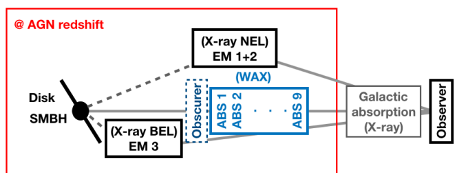
Fig. 12. Simplified view of the relations among spectral components observed in NGC 3783 in X-rays. Three different light paths are shown here. The obscurer (dashed box) is not always present along the line of sight. Dashed lines indicate that these photons are not directly observable. WAX is short for the warm absorber in X-rays. BEL and NEL refer to the broad and narrow emission lines. EM and ABS are short for emission and absorption, respectively.
