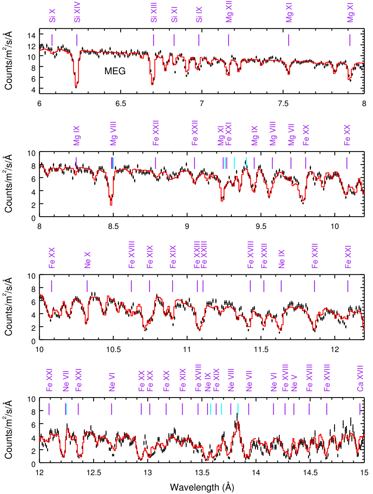
Fig. 3. The best-fit to the time-averaged MEG spectrum (in the observed frame) of NGC 3783 observed in 2000, 2001 and 2013. Most prominent absorption and emission features are labeled. The solid vertical lines in purple (blue) indicate the photoionized absorption (emission) features.
