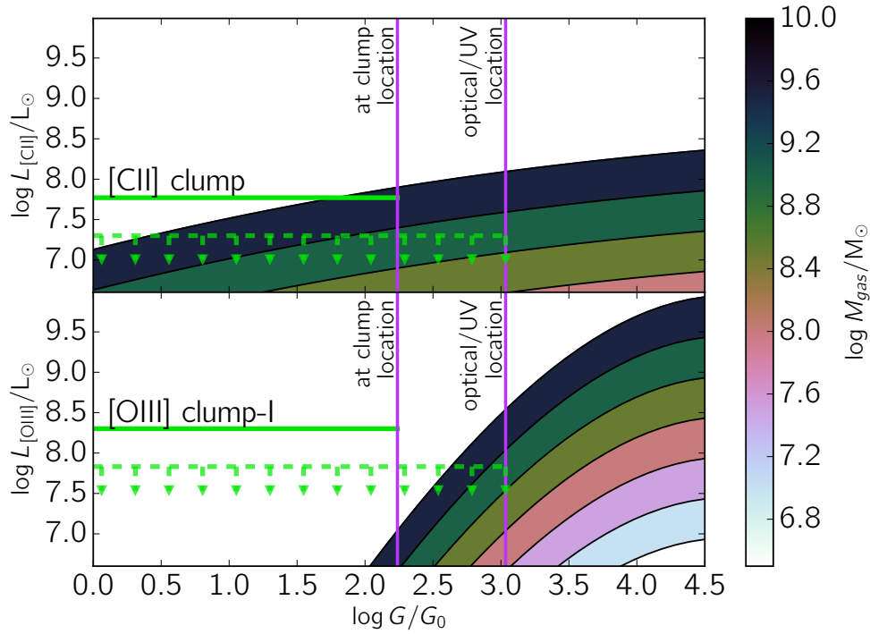
Fig. 7. Predicted [C II] (upper panel) and [O III] (lower panel) luminosities ( L ) as a function of the incident flux ( G ) exciting the line, inferred by using the model presented in V16, in which the colour shading is done according to M_{\text{gas}} , as encoded in the colourbar. In each panel we plot with a horizontal green line the luminosity inferred from our observations of the [C II] clump and of the [O III] clump-I. The horizontal dashed green lines show the upper limits at the location of the Y -band image of BDF-3299. Additionally, we show the flux G expected from BDF-3299 at the location of the [C II] and [O III] clumps and also the estimated average G within the galaxy BDF-3299. See the text for details.
