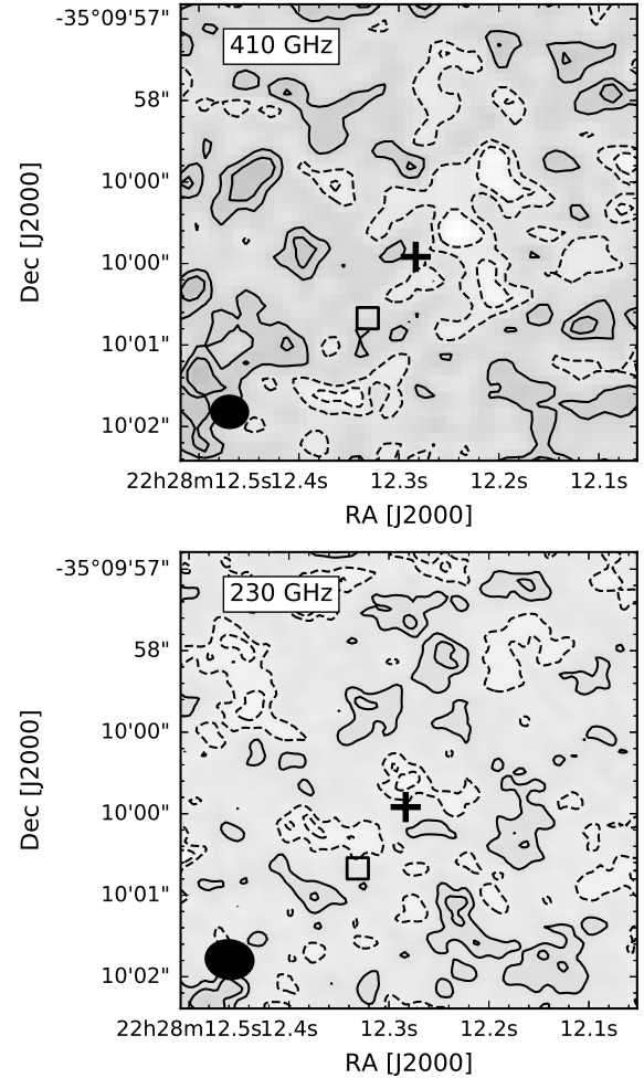
Fig. 1. ALMA continuum map in band 8 (410 GHz; top) and in Band 6 (230 GHz; bottom). Black solid contours are at levels of 1 and 2\sigma , where i.e \sigma = 40 \mu\text{Jy/beam} and \sigma = 7 \mu\text{Jy/beam} in the two bands, respectively. Dashed contours trace negative levels at -1 and -2\sigma . The synthesised beams are shown in the bottom left corners. The position of BDF-3299 measured in the HST Y -band is marked with a cross. The square mark shows the location of the [C II] detection.
