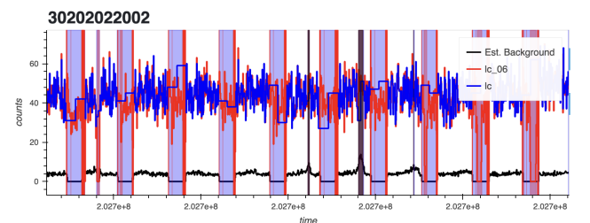
Figure 1. Example of the GTI cleaning process. The light curves shown (background and source) are constructed from the coadded FPMA + FPMB data, binned at \Delta t = 0.1 s. Intervals where the background exceeds 10% of the mean source level are excluded (black bands). Standard Earth-occultation or poor star-tracker intervals are shown with blue vertical bands, and data taken during limited star-tracker coverage are plotted in red (these red data are not used in PDS modeling).
