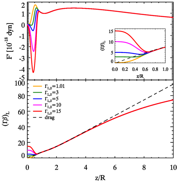
Figure 4. Radiative acceleration of the layer obtained by varying the initial layer Lorentz factor \Gamma_{L,0} = 1.01, 3, 5, 10, 15 . The spine isotropic luminosity is L_{\text{iso,S}} = 10^{45} \text{ erg s}^{-1} and the leptons of the layer are hot ( \langle \gamma_L^2 \rangle = 10^6 ) implying k_L = 10^{51} \text{ erg s}^{-1} . The spine Lorentz factor is constant \Gamma_S = 15 . Top panel: radiative force F' in the layer frame as a function of z/R . Bottom panel: layer Lorentz factor (\Gamma\beta)_L (solid lines) and the drag Lorentz factor (\Gamma\beta)_{L,\text{drag}} of the layer (dashed line) as a function of z/R . Inset: a zoomed view of the behaviour of the layer Lorentz factor for 0 < z/R < 1 .
