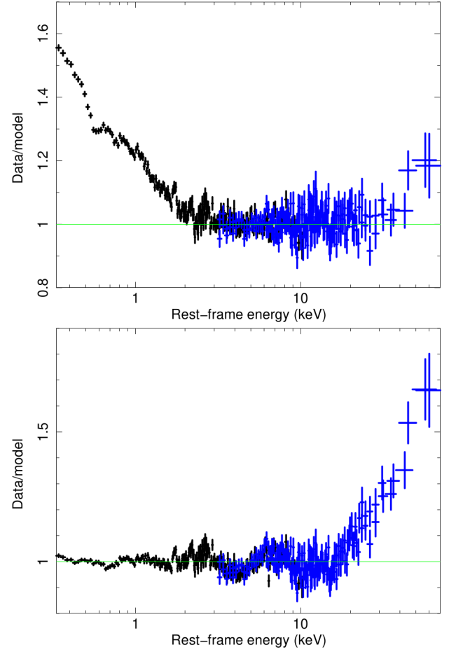
Fig. B.2. Residuals in term of data-to-model ratio for the fits of the 2022 simultaneous XMM-Newton -pn (black) and NuSTAR (blue) spectrum of ESO 141-G55 with the RELXILLCP model. Top panel: Fit above 3 keV (Table B.1), which has been extrapolated down to 0.3 keV. Bottom panel: Fit over the full 0.3–79 keV energy range.
