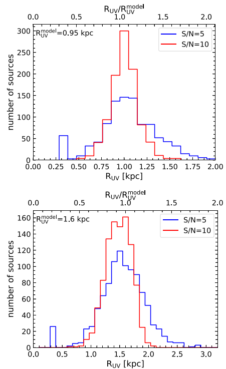
Figure B1. Distribution of the half-light radius R_{\text{UV}} estimated from 1000 simulated UV sources with \text{S/N} = 5 (blue histogram) and \text{S/N} = 10 (red histogram). Top and bottom panels show the results of the simulation for the two effective radii used in the model: R_{\text{UV}}^{\text{model}} = 0.95 \text{ kpc} and R_{\text{UV}}^{\text{model}} = 1.6 \text{ kpc} .
