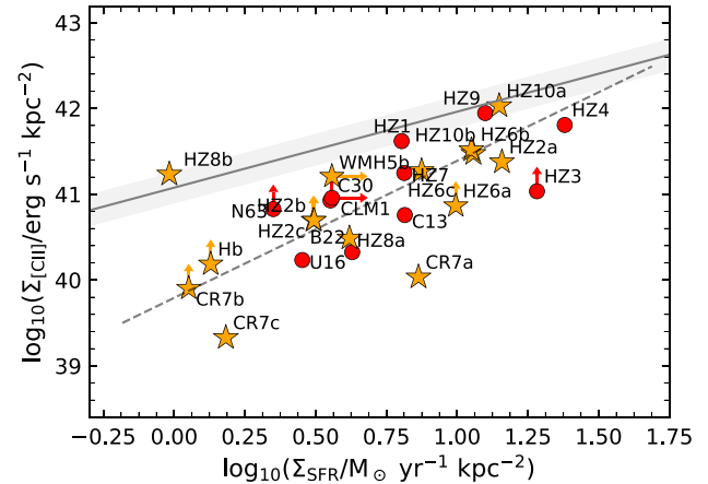
Figure 10. \Sigma_{[CII]} versus \Sigma_{SFR} for z > 5 star-forming galaxies detected both in [C II] and rest-frame UV. Symbols are as in Fig. 4. The grey line indicates the local relation by Herrera-Camus et al. (2015). The dashed line indicates the best linear fit on the z > 5 sample.
