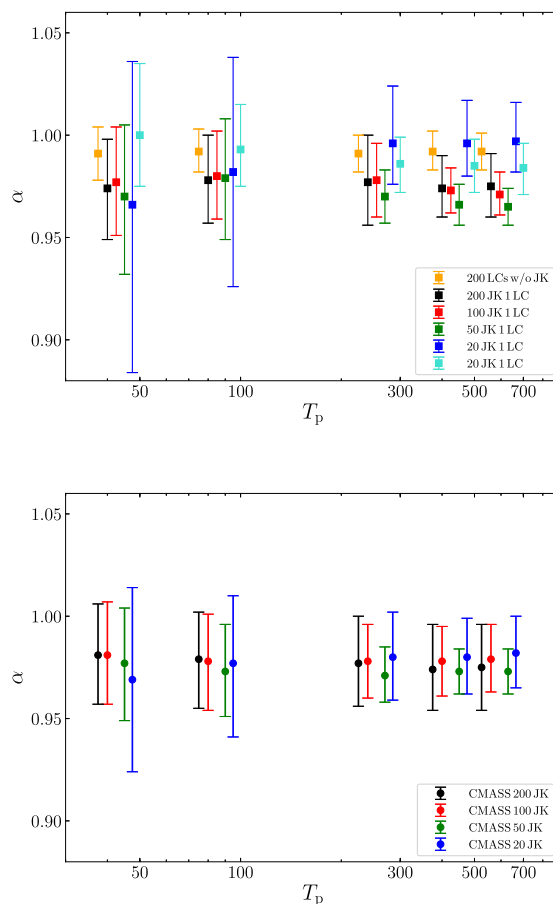
Figure 8. Shift parameter \alpha and its uncertainty as a function of the tapering parameter T_p . Top: Results from covariances computed from 200 LN mocks without jackknife and from jackknife performed on an LN realization. We have offset the T_p values on the x -axis by multiplying them, from left to right, by [0.75,0.80,0.85,0.90,0.95,1.0]. Bottom: results from CMASS jackknife resampling. The T_p values have been offset by multiplying them, from left to right, by [0.80,0.85,0.90,0.95,1.0].
