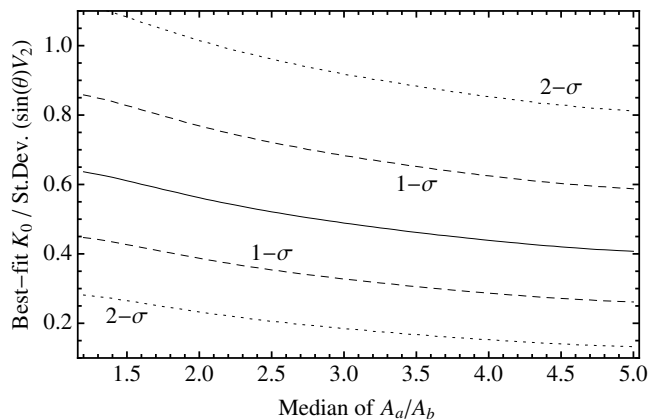
Figure 23. Dependence of the best-fit value of K_0 , scaled with the standard deviation of \sin(\theta)V_2 , on the spread of the A_a/A_b distribution.
