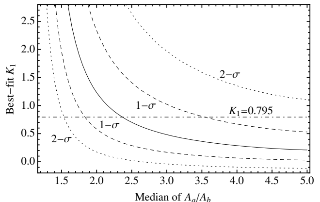
Figure 22. Dependence of the best-fit value of K_1 on the spread of the A_a/A_b distribution (expressed in terms of the median value of A_a/A_b , with A_a > A_b ).
