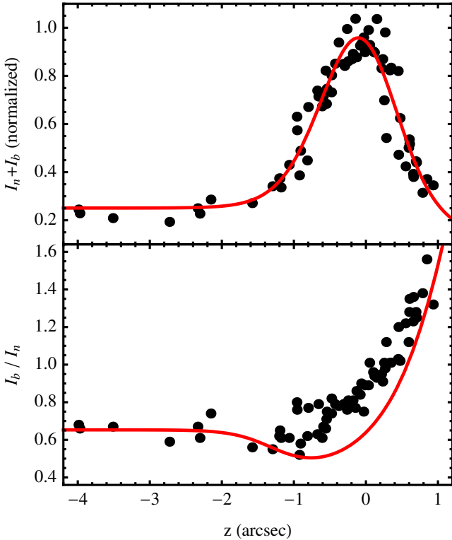
Figure 20. Simulated I_n + I_b and I_b/I_n profiles for the spatial resolution of N+13 (solid red lines), compared with actual observations in that work (black dots). The upper panel shows the result of the fit to the total line flux, needed to set the spatial resolution. The lower panel compares instead the prediction for the I_b/I_n profile, compared with the data.
