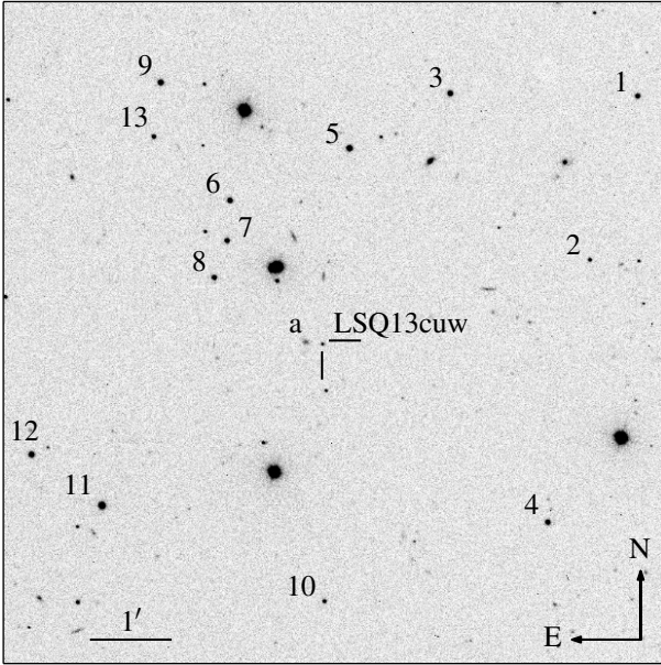
Fig. 1. LSQ13cuw and its environment. Short dashes mark the location of the supernova at \alpha_{J2000} = 02^{\text{h}}39^{\text{m}}57^{\text{s}}.35 , \delta_{J2000} = -08^{\circ}31'24''.2 . The nearest galaxy, marked “a”, originally presumed to be the host, is SDSS J023958.22-083123.5. The numbers mark the positions of the sequence stars (see also Table B.1) used for the photometric calibrations. r' -band image taken on 2013 November 29, 31.6 days after explosion.
