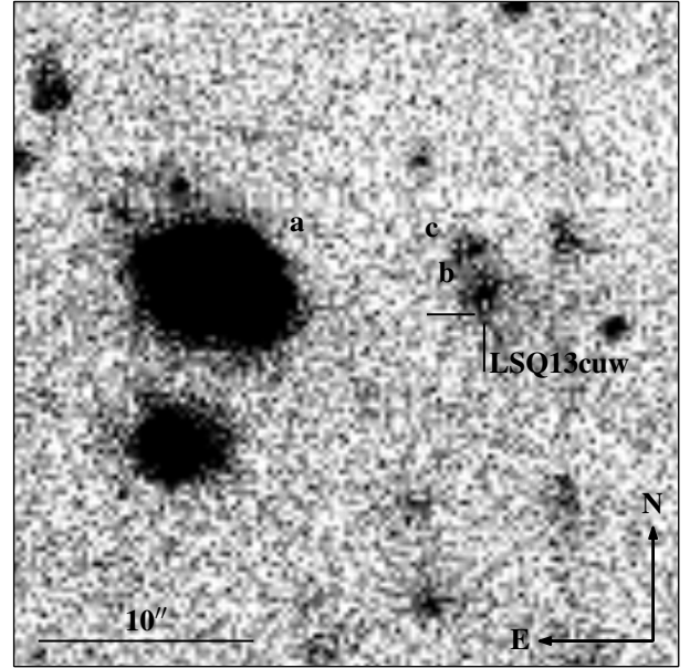
Fig. 3. Likely host galaxy of LSQ13cuw. A faint extended source was detected within 0'.5 of the reported position of SDSS J023957.37-083123.8, 1'3 NE from LSQ13cuw. The source appears elongated in the N–S direction with two bright regions at each end that are marked with “b” and “c”. “a” marks the position of the galaxy SDSS J023958.22-083123.5 that was originally presumed to be the host. Deep r' -band imaging obtained on 2014 September 24, 316.6 days after explosion (rest frame).
