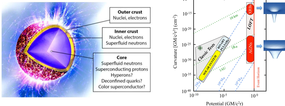
Figure 1. Left: Schematic structure of a neutron star. The outer layer is a solid ionic crust supported by electron degeneracy pressure. Neutrons begin to leak out of ions (nuclei) at densities \sim 4 \times 10^{11} \text{ g/cm}^3 (the neutron drip line, which separates inner from outer crust), where neutron degeneracy also starts to play a role. At densities \sim 2 \times 10^{14} \text{ g/cm}^3 , the nuclei dissolve completely. This marks the crust-core boundary. In the core, densities may reach up to ten times the nuclear saturation density of 2.8 \times 10^{14} \text{ g/cm}^3 (the density in normal atomic nuclei). (Graphics credit: NASA). Right: LOFT probes the deepest gravitational wells in the Universe: BHs. Current GR tests use potentials 10^4 times lower. LOFT uniquely covers a factor 10^{16} in spacetime curvature with uniform diagnostics.
