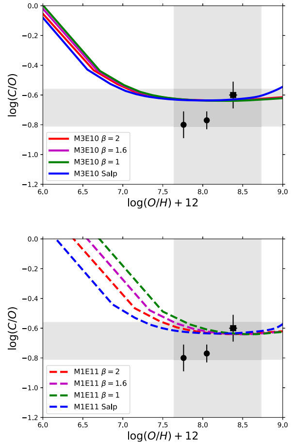
Figure 7. \log(C/O) versus \log(O/H)+12 computed without taking into account dust depletion and compared with abundances measured in galaxies of the sample of Table 3. Upper panel: lines are computed for M3E10 models (solid) with Salpeter (1955) IMF (blue) and W11 IGIMF calculated for \beta = 1 (green), \beta = 1.6 (magenta) and \beta = 2 (red). Lower panel: lines are computed for M1E11 models (dashed) with Salpeter (1955) IMF (blue) and W11 IGIMF calculated for \beta = 1 (green), \beta = 1.6 (magenta), and \beta = 2 (red). For both panels: the shaded regions indicate the \log(C/O) confidence region derived from the composite LBG spectrum of Shapley et al. (2003) and the \log(O/H)+12 characterizing the sample of LBGs of Pettini et al. (2001). Other data are from Steidel et al. (2016) stacked spectrum (filled square), Bayliss et al. (2014) and Christensen et al. (2012a,b) (filled circles).
