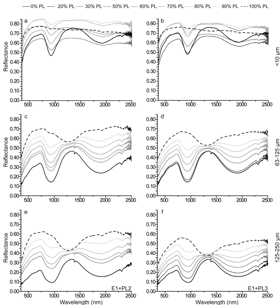
Fig. 2. Reflectance spectra of E1-PL mixtures at three different particle sizes. (a, b) E1+PL2 and E1+PL3, <10\ \mu\text{m} ; (c, d) E1+PL2 and E1+PL3, 63\text{--}125\ \mu\text{m} ; and (e, f) E1+PL2 and E1+PL3, 125\text{--}250\ \mu\text{m} . Generally, a fine particle size produces spectra with higher reflectance and reduced spectral contrast compared to the coarsest sizes.
