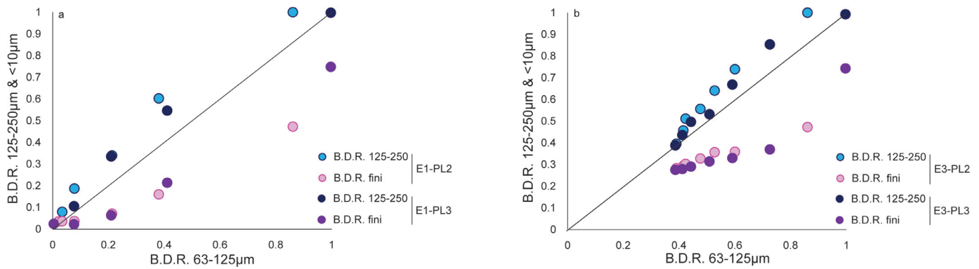
Fig. 10. Band Depth Ratio (B.D.R.) for the 125–250 μm and <10 μm sizes vs. the 63–125 μm size. (a) E1-bearing mixtures; (b) E3-bearing mixtures. The bisector indicates the ideal conditions that the relative depths do not change with the size; however, 125–250 μm values (blue symbols) stay above the line, while <10 μm values (magenta symbols) are under the line. (For interpretation of the references to colour in this figure legend, the reader is referred to the web version of this article.)
