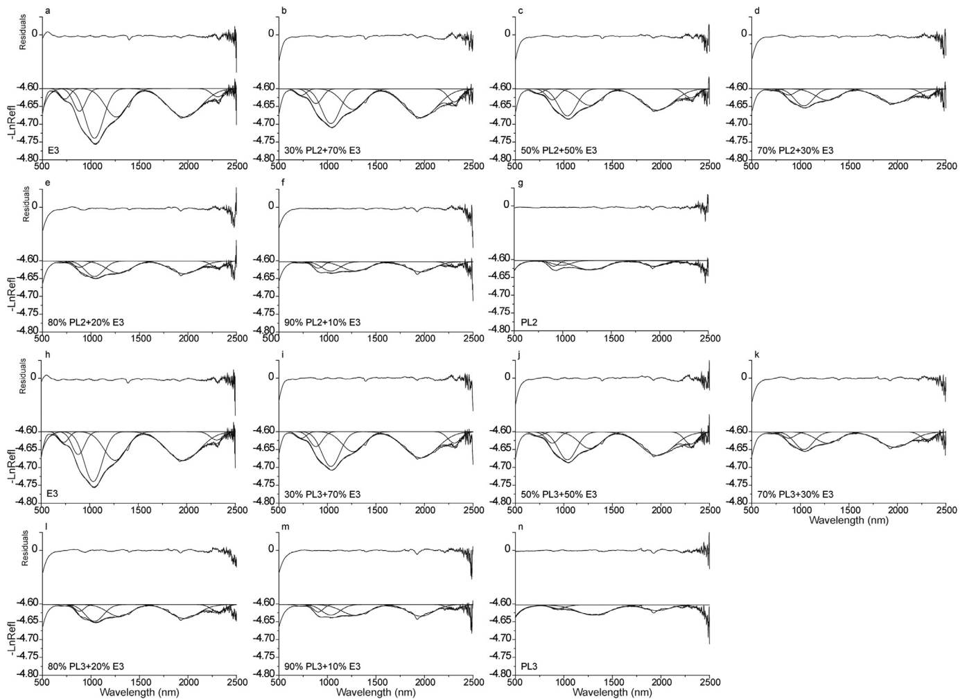
Fig. 6. MGM deconvolution and residuals of E3-bearing mixtures. RMS values are consistent with Klima et al. (2011). (a–g) E1-PL2 mixtures; (h–n) E1-PL3 mixtures. Continuum-removed reflectance is expressed as -\text{LnRefl} .
