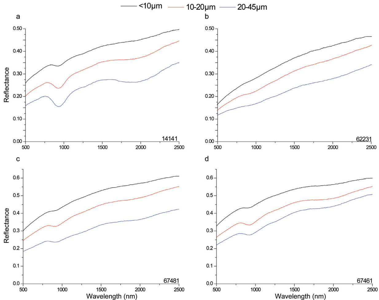
Fig. 11. Spectra of lunar soils (from the Lunar Soil Characterization Consortium, from Pieters et al. (1993, 2000) at three different, very fine particle sizes (20–45 μm blue spectra, 10–20 μm red spectra and <10 μm black spectra). Samples #67,481 and #67,461 are more enriched in PL than samples #14,141 and #62,231. Generally, reducing the size the reflectance increases, absorption bands are shallower and, in particular, the 1250 nm band becomes almost featureless in <10 μm spectra. (For interpretation of the references to colour in this figure legend, the reader is referred to the web version of this article.)
