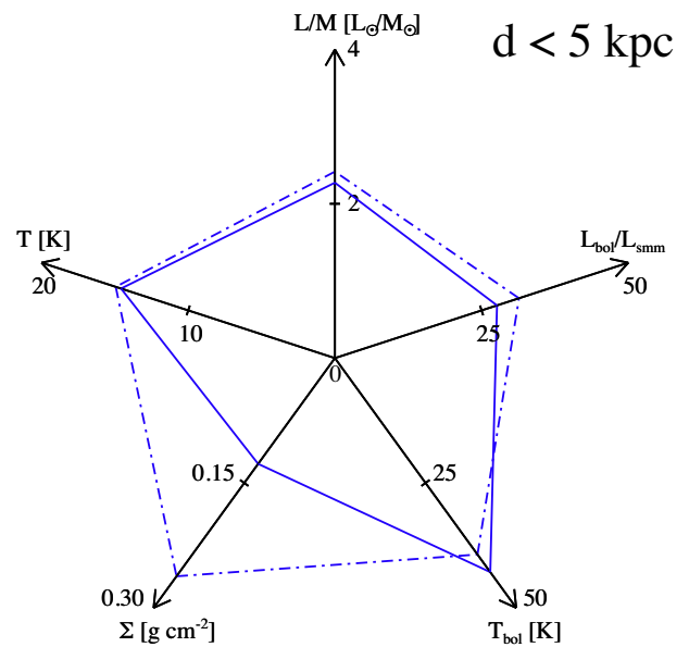
Figure 27. Same as Fig. 26, but for the subset of protostellar sources within heliocentric distance d < 5\ \text{kpc} .
