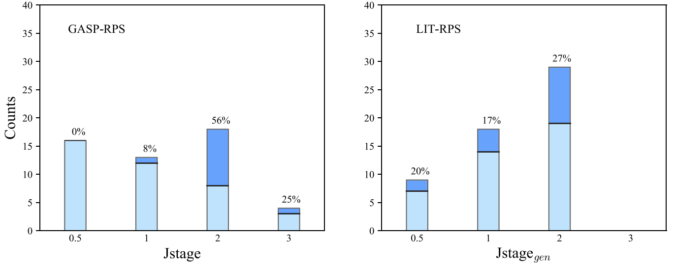
Figure 3. Stacked histograms for galaxies of different Jstages and divided among centrally star-forming galaxies (light blue histogram) and AGNs (dark blue histogram) according to the BPT-N II classification for GASP-RPS (left) and LIT-RPS (right). Percentages are AGN fractions in the corresponding bin of Jstage and Jstage gen .
