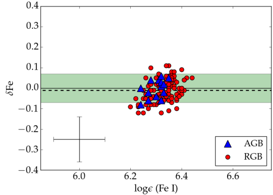
Figure 4. Fe abundances for this study. Here, ionisation difference ( \delta\text{Fe} = \log_\epsilon(\text{Fe I}) - \log_\epsilon(\text{Fe II}) ) is plotted against \log_\epsilon(\text{Fe I}) abundance to highlight departures from LTE in Fe I, and the similarity between the Fe abundances of the AGB and RGB. The error bar indicates typical 1\sigma total uncertainties in individual abundances (i.e. the line-to-line uncertainties and the 1\sigma atmospheric sensitivity uncertainties added in quadrature), while the black dashed line represents the sample average \delta\text{Fe} value of -0.01 . The shaded green region indicates the non-LTE uncertainties quoted in Amarsi et al. (2016b) , \pm 0.05 dex, around the expected \delta\text{Fe} value ( +0.00 dex, solid black line) from our non-LTE test (see §2.3).
