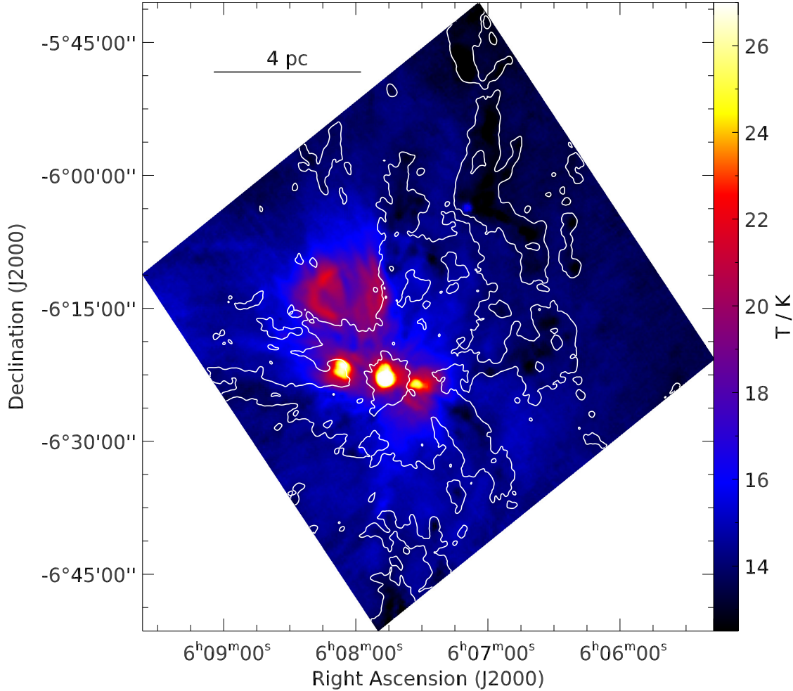
Fig. 4. Monoceros R2 dust temperature map. The resolution is as for the 500\ \mu\text{m} map ( 36.4'' ). The contours (as for Fig. 3) are at the \text{H}_2 column densities 7.5 \times 10^{21}\ \text{cm}^{-2} and 3.5 \times 10^{22}\ \text{cm}^{-2} .
