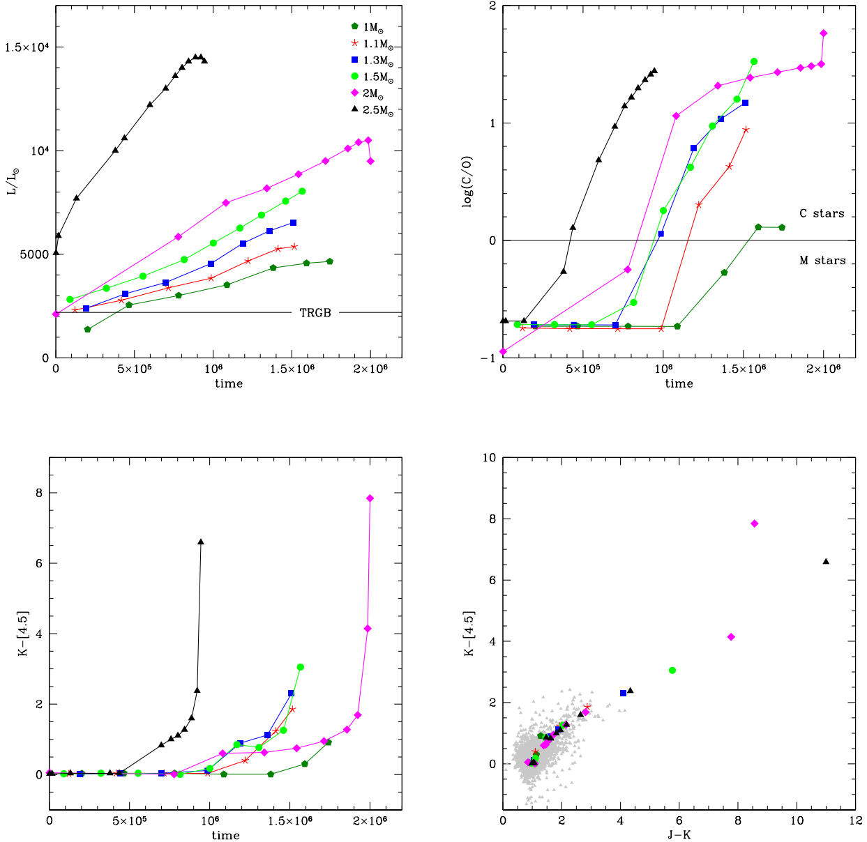
Figure 2. The evolution of the luminosity (top, left panel) and of the C/O ratio (top, right) of 1-2 M_{\odot} at Z = 10^{-3} and 2.5 M_{\odot} at Z \leq 2 \times 10^{-3} . The thin, horizontal lines mark the location of the TRGB and the boundary between M stars and carbon stars. The variation of the (K-[4.5]) colour is shown in the bottom, left panel. We also show the excursion of the tracks in the colour-colour ( J-K ) vs ( K-[4.5] ) plane, overimposed to the data of the IC10 evolved stellar population by Gerbrandt et al. (2015) and Boyer et al. (2015a). The adopted reddening is E(B - V) = 1.14 mag (see section 5.2)
