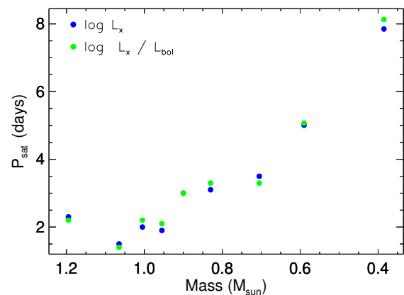
Fig. 7. Rotation period at which the saturation level ( P_{\text{sat}} ) as a function of the stellar mass is reached. The blue and green dots correspond with the rotation period value at which the saturation occurs in L_x and L_x/L_{\text{bol}} representation, respectively.
