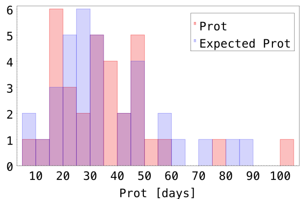
Fig. 2. Distribution of the rotation periods for the stars in our sample. The red area shows the measured rotation periods and the blue area corresponds to the derived rotation periods when a direct determination was not possible.
