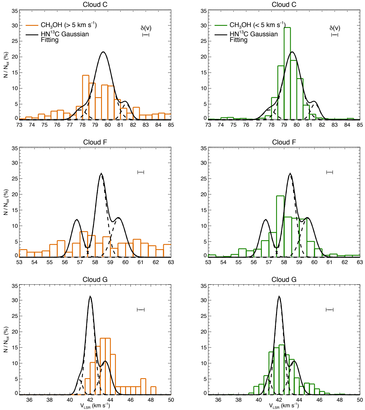
Figure 10. Velocity distribution of the \text{CH}_3\text{OH} broad (linewidths > 5 \text{ km s}^{-1} , orange in left panels) and narrow (linewidths < 5 \text{ km s}^{-1} , green in right panels) emission obtained for clouds C (top panels), F (middle panels) and G (bottom panels). The histograms show the percentage of emission lines having radial velocities falling within each bin, with bin sizes 0.5 \text{ km s}^{-1} for the three clouds, corresponding to 1/3 of the mean intensity-weighted linewidth obtained for the dense gas tracers. The contribution from all \text{CH}_3\text{OH} transitions detected in each cloud has been considered. In each panel, the mean uncertainty for the central velocities of the single fittings is indicated. Black curves correspond to the gaussian fitting obtained for \text{HN}^{13}\text{C} in Section 4.1.1 (see also Figure 3).
