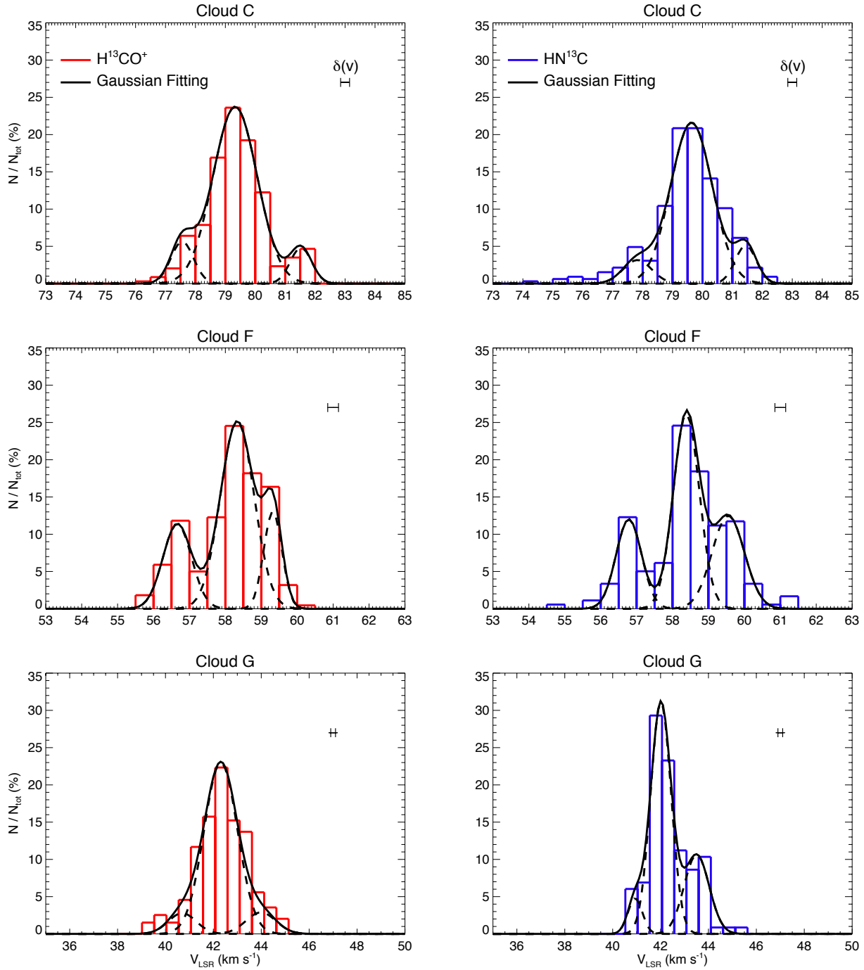
Figure 3. Velocity distributions of the \text{H}^{13}\text{CO}^+ (red) and \text{HN}^{13}\text{C} (blue) emissions as obtained for cloud C (top panel), cloud F (middle panel) and cloud G (bottom panel). The histograms show the percentage of emission lines having V_{\text{LSR}} falling within the \delta V of the bin. Bin sizes are 0.5 \text{ km s}^{-1} for the three clouds, which corresponds to 1/3 of mean intensity-weighted linewidth for the two tracers. In all panels the mean uncertainty in the central velocities of the fittings is indicated.
