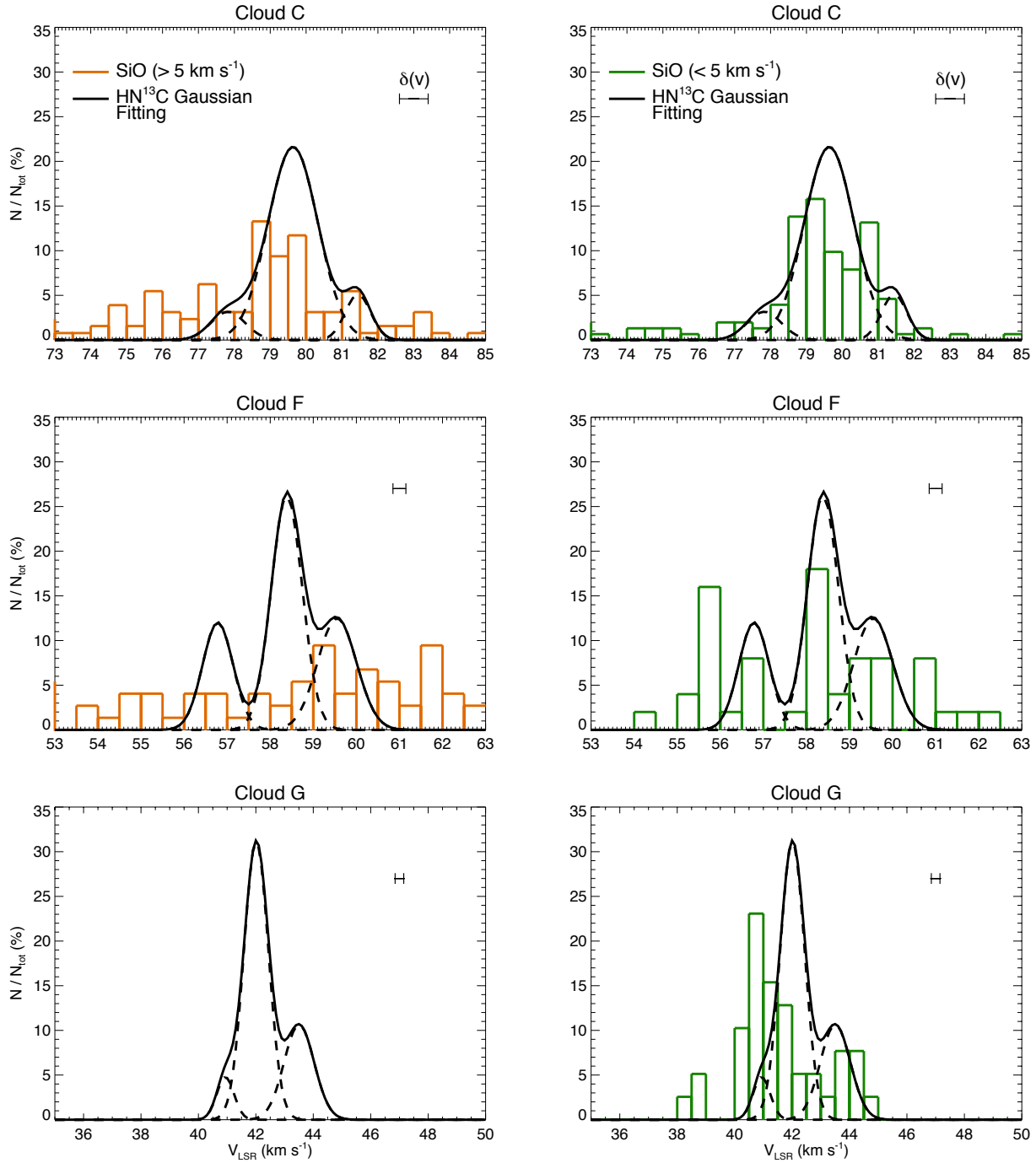
Figure 9. Velocity distribution of the SiO broad (with linewidths >5 \text{ km s}^{-1} , orange in left panels) and narrow (with linewidths <5 \text{ km s}^{-1} , green in right panels) emission obtained for cloud C (top panels), F (middle panels) and G (bottom panels). The histograms show the percentage of emission lines having radial velocities falling within each bin, where the bin size is 0.5 \text{ km s}^{-1} for the three clouds, corresponding to 1/3 of the mean intensity-weighted linewidth obtained for the dense gas tracers. In each panel, the mean uncertainty for the central velocities of the single fittings is indicated. Black curves correspond to the gaussian fitting obtained for \text{HN}^{13}\text{C} in Section 4.1.1 (see also Figure 3).
