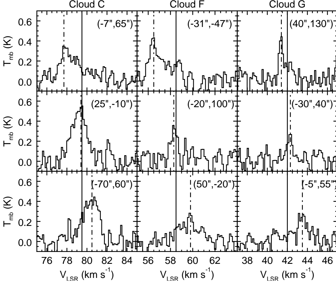
Figure 2. \text{HN}^{13}\text{C} spectra for clouds C (left panel), F (middle panel) and G (right panel) extracted toward several positions and highlighting the presence of multiple velocity components. The vertical solid lines correspond to the central velocity of the clouds while the vertical dot-dashed lines indicate the central velocity of the spectrum peaks. The same result has been found for the \text{H}^{13}\text{CO}^+ emission in all the three clouds and are not shown for simplicity.
