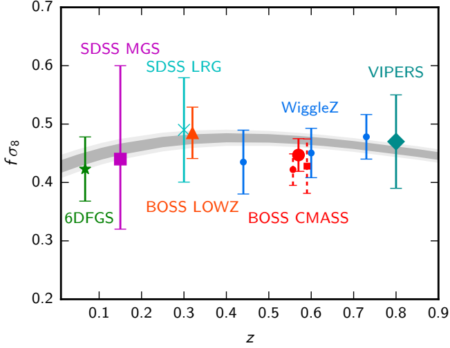
Fig. 16. Constraints on the growth rate of fluctuations from various redshift surveys in the base \Lambda CDM model: green star (6dFGS, Beutler et al. 2012); purple square (SDSS MGS, Howlett et al. 2015); cyan cross (SDSS LRG, Oka et al. 2014); red triangle (BOSS LOWZ survey, Gil-Marín et al. 2015); large red circle (BOSS CMASS, as analysed by Samushia et al. 2014); blue circles (WiggleZ, Blake et al. 2012); and green diamond (VIPERS, de la Torre et al. 2013). The points with dashed red error bars correspond to alternative analyses of BOSS CMASS from Beutler et al. (2014, small circle, offset for clarity) and Chuang et al. (2013, small square). Of the BOSS CMASS points, two are based on the same DR11 data set (Samushia et al. 2014; Beutler et al. 2014), while the third is based on the more recent DR12 (Chuang et al. 2013), and are therefore not independent. The grey bands show the range allowed by Planck TT+lowP+lensing in the base \Lambda CDM model. Where available (for SDSS MGS and BOSS), we have plotted conditional constraints on f\sigma_8 assuming a Planck \Lambda CDM background cosmology. The WiggleZ points are plotted conditional on the mean Planck cosmology prediction for F_{\text{AP}} (evaluated using the covariance between f\sigma_8 and F_{\text{AP}} given in Blake et al. 2012). The 6dFGS point is at sufficiently low redshift that it is insensitive to the cosmology.
