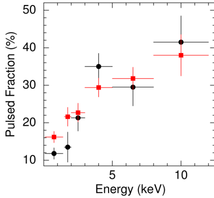
Figure 2. Background subtracted pulsed fractions of the 0.42-s signal as a function of energy for the 2013 (circles) and 2014 (squares) pn data.
