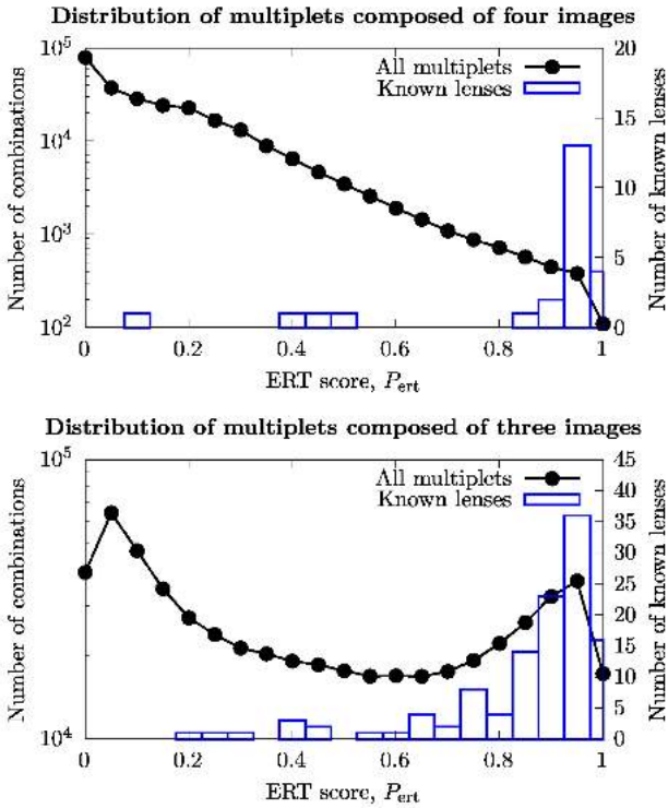
Fig. 10. Distribution of the ERT scores for the 56 398 multipliets (24 known lenses) composed of at least four components (top) and 134 656 multipliets (45 known lenses) composed of at least three components (bottom). If multipliets are composed of more than three or four components, respectively, then all combinations of three and four components are considered for computing the ERT scores.
