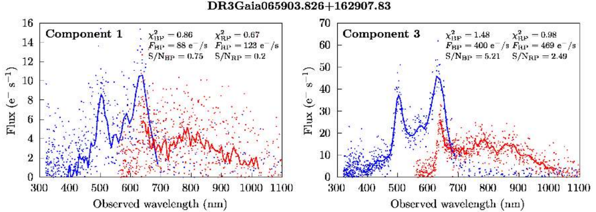
Fig. 11. Epoch and resampled BP and RP spectra of the first and third components of the quadruple lens system GraL J065904.1+162909 (Delchambre et al. 2019; Stern et al. 2021), corresponding to the GravLens multiplet DR3Gaia065903.826+162907.83. Points are the epoch BP/RP spectra of each of the components (blue for BP, red for RP) while solid lines are the resampled BP/RP spectra, as described in Sect. 5.3. We also provide the additional parameters derived during the resampling phase: mean resampling chi-square ( \chi^2_{XP} ), integrated flux ( F_{XP} ) and signal-to-noise ratio ( S/N_{XP} ) where XP stands for BP or RP. Both component spectra show strong Ly \alpha and C IV emission lines that allow us to unambiguously identify this multiplet as a lensed QSO.
