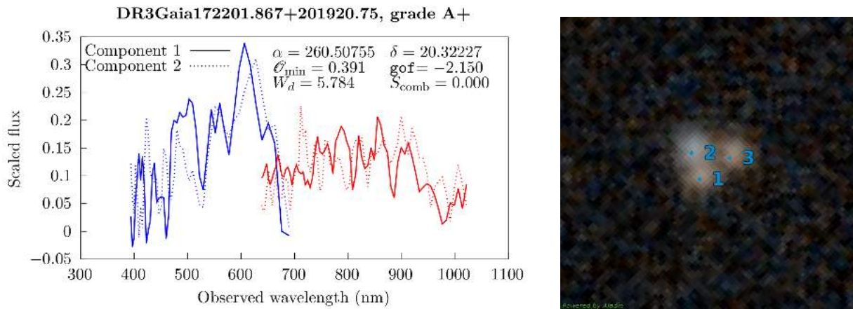
Fig. B.33. Comparison of the resampled spectra of the DR3Gaia172201.867+201920.75 multipler (Left) and associated Pan-STARRS1 image (Right) (Chambers et al. 2016). Blue dots correspond to the GravLens components. The cutout size is 15.0'' \times 15.0'' , north is up and east is left.
