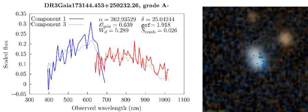
Fig. B.34. Comparison of the resampled spectra of the DR3Gaia173144.453+250232.26 multipler (Left) and associated Pan-STARRS1 image (Right) (Chambers et al. 2016). Blue dots correspond to the GravLens components. The cutout size is 15.0'' \times 15.0'' , north is up and east is left.
