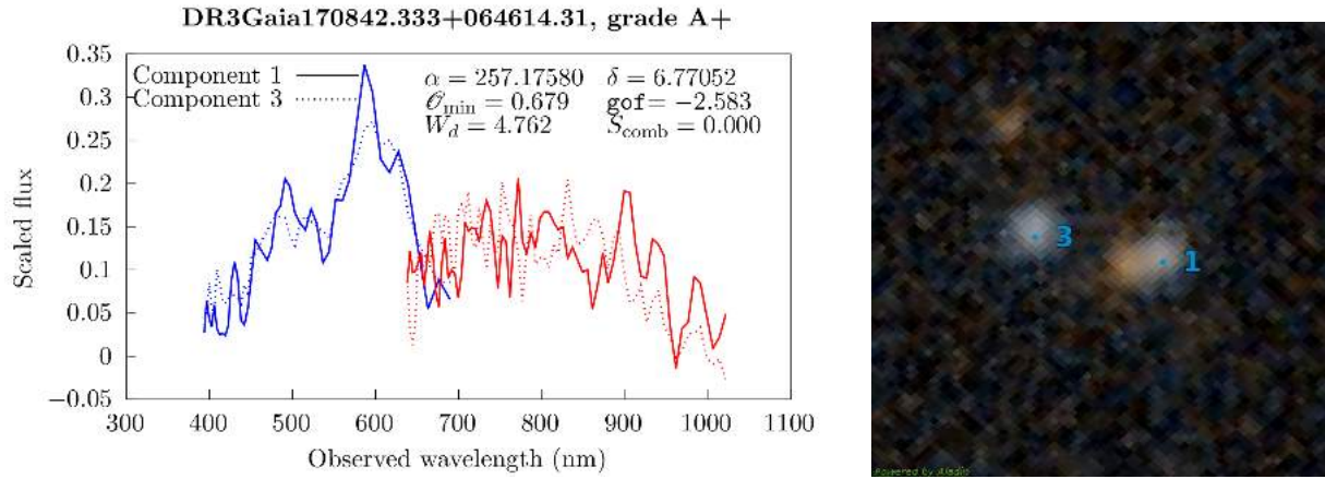
Fig. B.32. Comparison of the resampled spectra of the DR3Gaia170842.333+064614.31 multipler (Left) and associated Pan-STARRS1 image (Right) (Chambers et al. 2016). Blue dots correspond to the GravLens components. The cutout size is 15.0'' \times 15.0'' , north is up and east is left.
