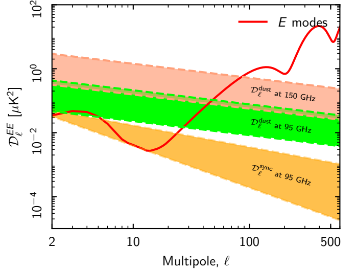
Fig. 11. Dust and synchrotron E -mode power versus multipole. The dust power at 95 and 150 GHz and that of synchrotron at 95 GHz are compared with the CMB E -mode signal (red-line) computed for the Planck 2015 \Lambda CDM model (Planck Collaboration XIII 2016) and a Thompson scattering optical depth \tau = 0.055 from Planck Collaboration Int. XLVI (2016). The coloured bands show the range of power measured in our analysis. The lower limit of the synchrotron band is derived from the S-PASS data analysis in Krachmalnicoff et al. (2018).
