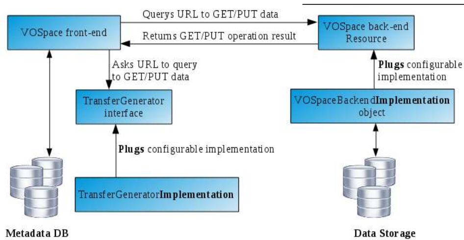
Figure 2. VOSpace architectural base.
