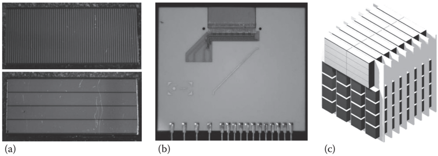
FIGURE 4.11 (a) Drift-strip CZT sensor ( 18 \times 8 \times 2.5 \text{ mm}^3 ): (top) anode side with a set of 64 (0.15 mm wide) strips, (bottom) cathode side with four (2 mm wide) strips. (b) Linear module prototype seen from the anode side: this constitutes the basic element for building a large-volume 3-D sensor. (c) A suitable packaging scheme of eight linear modules, each supporting two CZT drift 3-D sensors of 20 \times 20 \times 5 \text{ mm}^3 to obtain a spectroscopic imager of 32 \text{ cm}^3 sensitive volume.
