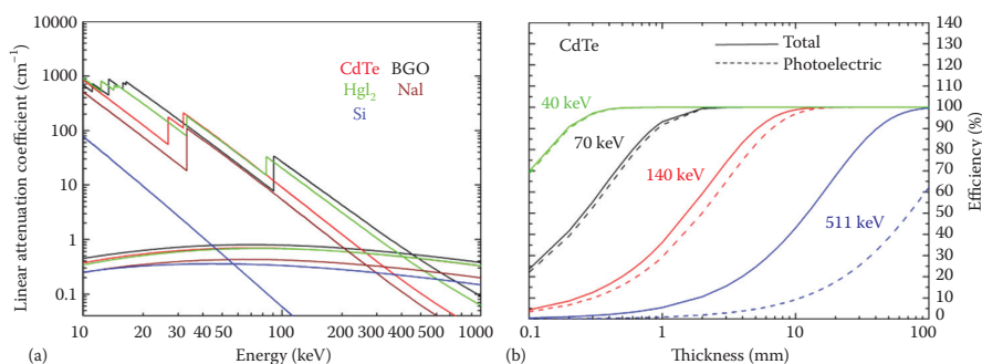
FIGURE 4.1 (a) Linear attenuation coefficients for photoelectric absorption and Compton scattering of CdTe, Si, HgI 2 , NaI, and BGO. (b) Efficiency of CdTe detectors as a function of detector thickness at various photon energies.
