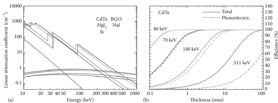
FIGURE 4.1 (See color insert) (a) Linear attenuation coefficients for photoelectric absorption and Compton scattering of CdTe, Si, \text{HgI}_2 , NaI, and BGO. (b) Efficiency of CdTe detectors as a function of detector thickness at various photon energies.
