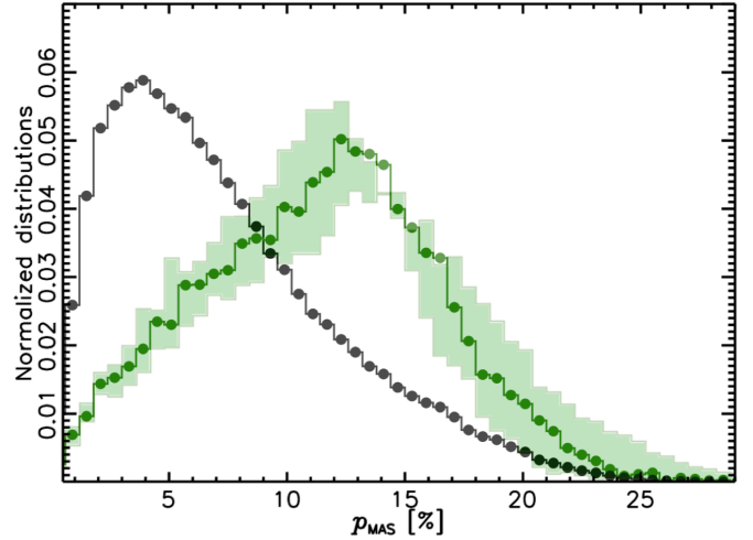
Fig. 3. Normalized distributions of the polarization fraction from the p_{\text{MAS}} debiased estimator (see text). The black distribution shows p_{\text{MAS}} over the whole sky. The green distribution shows p_{\text{MAS}} at b < -60^\circ . The green-shaded area represents the 1\sigma error on p_{\text{MAS}} at high latitude.
