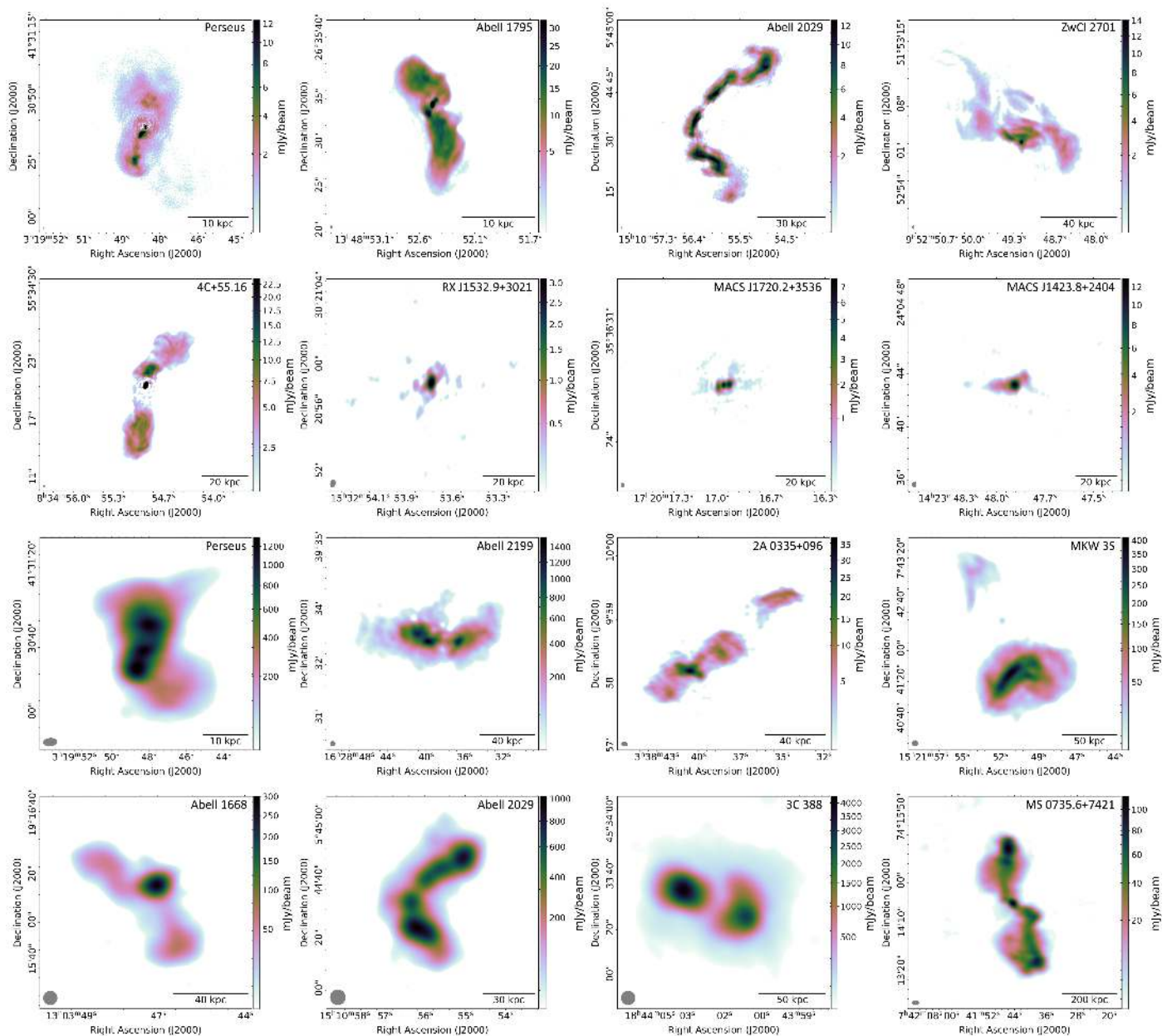
Fig. 1. LOFAR images of all galaxy clusters our the sample. The top 8 panels show the high-resolution maps produced by including LOFAR’s international stations and the bottom 8 panels show the low-resolution maps produced using only the Dutch part of the array. Note that Perseus and Abell 2029 are presented in both sections. The central dominant compact component in the Perseus cluster was peeled from the data for the low-resolution map for calibration purposes. The color maps range from three times the rms noise level to the peak brightness, except in the cases of Perseus, Abell 1795 and 4C+55.16, for which the peak brightness of the lobes was used due to the otherwise dominant central compact component. The scale bar in the bottom right corner of each panel measures the listed length at the redshift of the respective clusters. The beam is indicated in grey in the bottom left corner of each panel.
