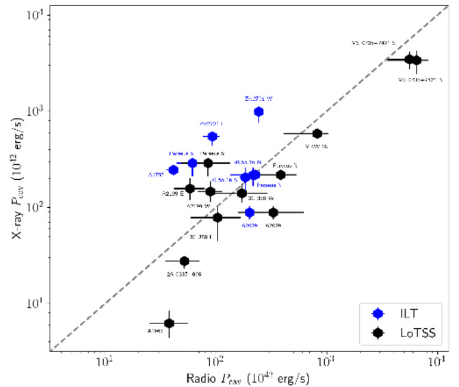
Fig. 5. The hybrid X-ray–radio cavity power measurements versus the purely X-ray-based cavity power estimates. The blue data points indicate the measurements derived using high-resolution observations, while the black data points indicate the measurements derived using low-resolution observations.
