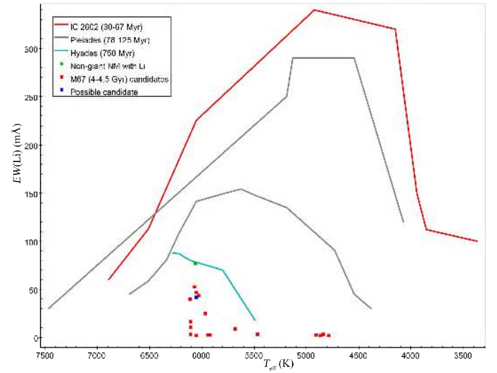
Fig. B.78. EW(Li) -versus- T_{\text{eff}} figure for M67.
