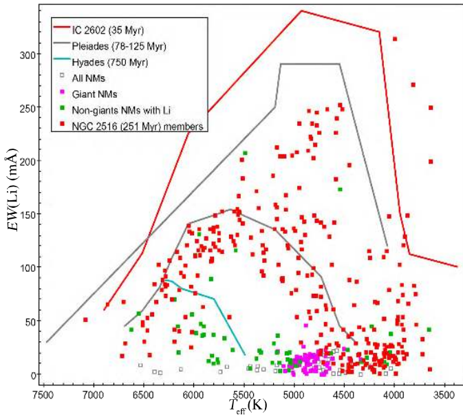
Fig. B.34. EW(\text{Li}) -versus- T_{\text{eff}} figure for NGC 2516.
