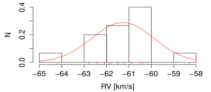
Fig. B.49. Gaussian fit of the RV distribution for the final selection of Trumpler 23.
