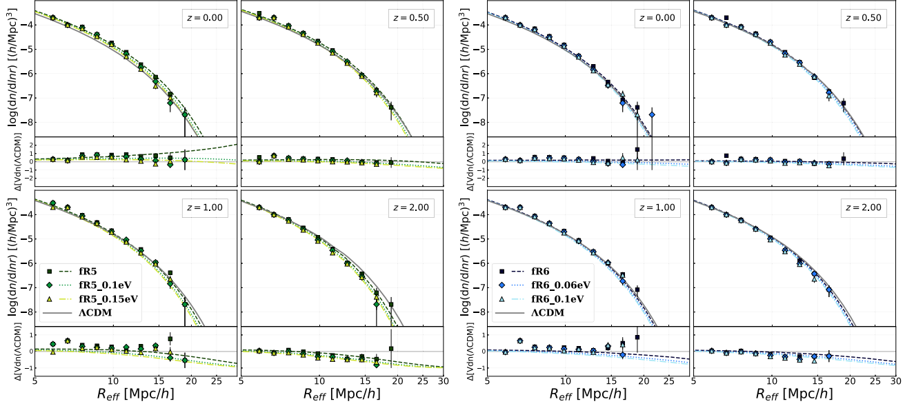
Figure 5. Measured and theoretical void size function computed at redshifts z = 0, 0.5, 1 , and 2 for the models fR5, fR5_0.1eV, fR5_0.15eV (left-hand panels) and fR6, fR6_0.06eV, fR6_0.1eV (right-hand panels). The description of these plots is analogous to the one reported in the caption of Fig. 4.
