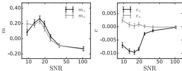
Figure 7. The multiplicative ( m_+ , m_\times ) and additive ( c_+ , c_\times ) biases of the measured shapes as a function of SNR. The bias components are derived by aligning the galaxy’s ellipticity and shear to the corresponding PSF ellipticity.
