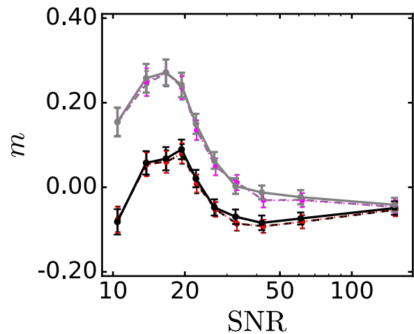
Figure 12. The multiplicative bias as a function of SNR. The black and grey dashed lines represent the two bias components m_1 and m_2 derived from the entire simulation sample, while the solid lines are the corresponding components after rejecting the neighbouring galaxies. The dotted lines indicate the average bias derived from the subsamples of galaxies by repeated sampling 100 times.
