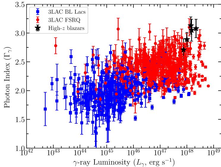
Figure 1. Photon index vs. \gamma -ray luminosity plane for 3LAC and high-redshift blazars at z > 3.1 detected in \gamma rays. Adapted from Ackermann et al. (2017)
