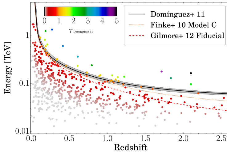
Figure 2. The highest-energy photons vs. redshift for 3FHL blazars, color coded by the optical depth calculated from the model presented by Domínguez et al. (2011). The cosmic \gamma -ray horizon based on different EBL models is shown. Adapted from Ajello et al. (2017)
