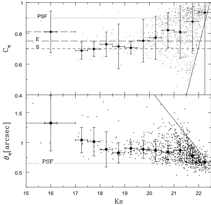
Fig. 7. Compactness index C_\eta (upper panel) and apparent size \theta_{0.5} (lower panel) as a function of Ks magnitude. The filled (red) circles are the median values in a 0.5 mag bin width. Vertical error bars are the standard deviation in each magnitude bin while horizontal bars represent the bin width. The dotted, the dashed and the long-dashed lines in the upper panel indicate the values of C_\eta for PSF, Spiral and Elliptical profiles respectively (see Sect. 5.2). The solid line in the lower panel shows the magnitude enclosed in an aperture of radius \theta and a uniform surface brightness Ks=22.76 mag/arcsec 2 while the dotted line represent the characteristic size of a point source in our images.
