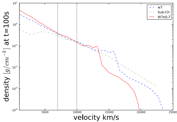
Figure 8. The W7, Sub-Ch and W7e0.7 density profiles as a function of velocity at t = 100 s after explosion. The vertical grey lines show the range in values v_{\text{ph}} can take, for the -3 d to +2 d models.
