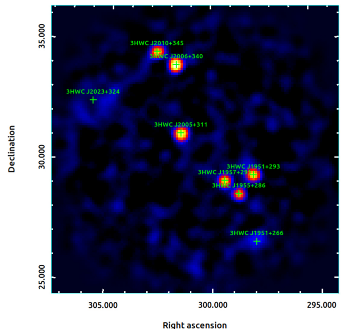
Fig. 13. ASTRI Mini-Array 200 hr simulation of the Cygnus Region. Green crosses mark the positions of the 3HWC sources in a 10^\circ \times 10^\circ field of view (see text for details).
