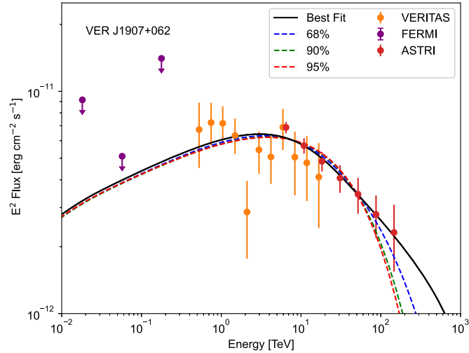
Fig. 18. VER J1907+062: \gamma -ray data from Fermi (Acero et al., 2013) (purple dots), VERITAS (Aliu et al., 2014) (orange dots) and ASTRI Mini-Array simulations for 100h of observations (red dots). The blue, green and red lines show the broken power law fit with a cut-off energy of 1.67, 0.54 and 0.4 PeV, corresponding to 68%, 90% and 95% of confidence level respectively. The ASTRI Mini-Array spectral points and their error bars are obtained from the distribution of 100 simulations. See text for more details.
