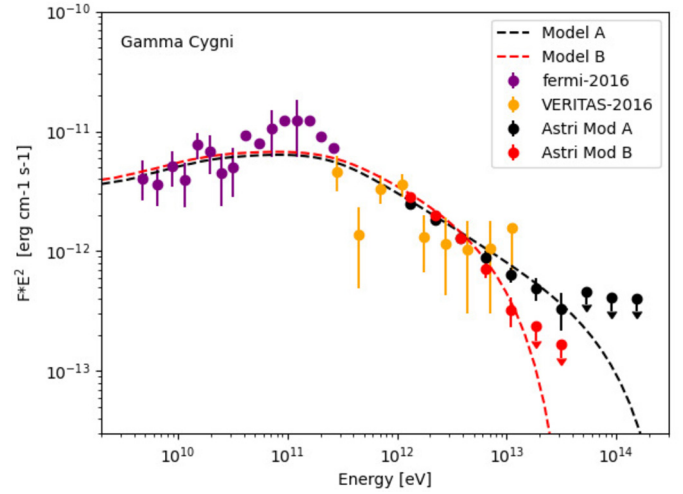
Fig. 20. \gamma -ray spectrum of \gamma -Cygni. Data are from Fermi-LAT and VERITAS while theoretical models A and B (described in the text) are showed with dashed curves. Black and red dots show the ASTRI Mini-Array simulations for model A and B, respectively, for 200 hr of exposure.
