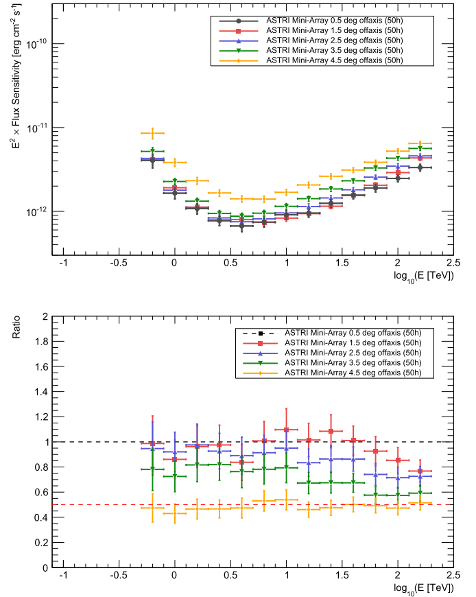
Fig. 8. Top: Off-axis differential sensitivity (multiplied by energy squared) of the ASTRI Mini-Array as a function of the energy between 10^{-0.3} \simeq 0.5 TeV and 10^{2.3} \simeq 200 TeV for 5 source off-axis bins between 0^\circ and 5^\circ . 50 hours of observations are considered. Bottom: Differential sensitivity ratios with respect to the differential sensitivity achieved in the first considered off-axis bin (from 0^\circ to 1^\circ ). The ratio is calculated so that higher values correspond to better performance. The dashed, thin red line represents a performance drop of a factor 2.
