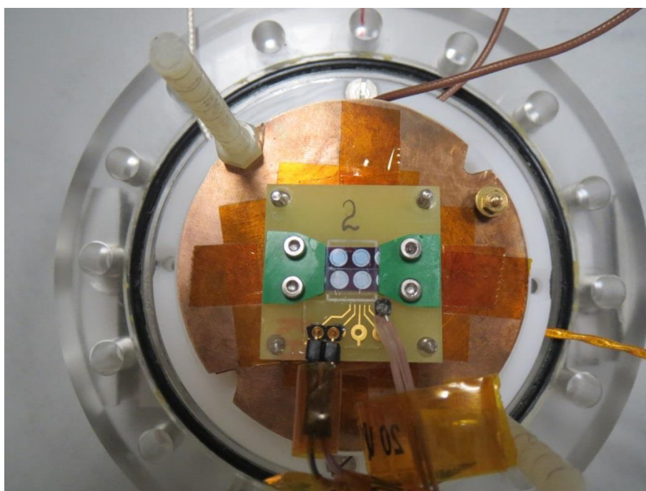
Figure 81: Picture of a set of diodes mounted on the flange of the small experimental chamber at the Cosmic Dust Accelerator Facility.
