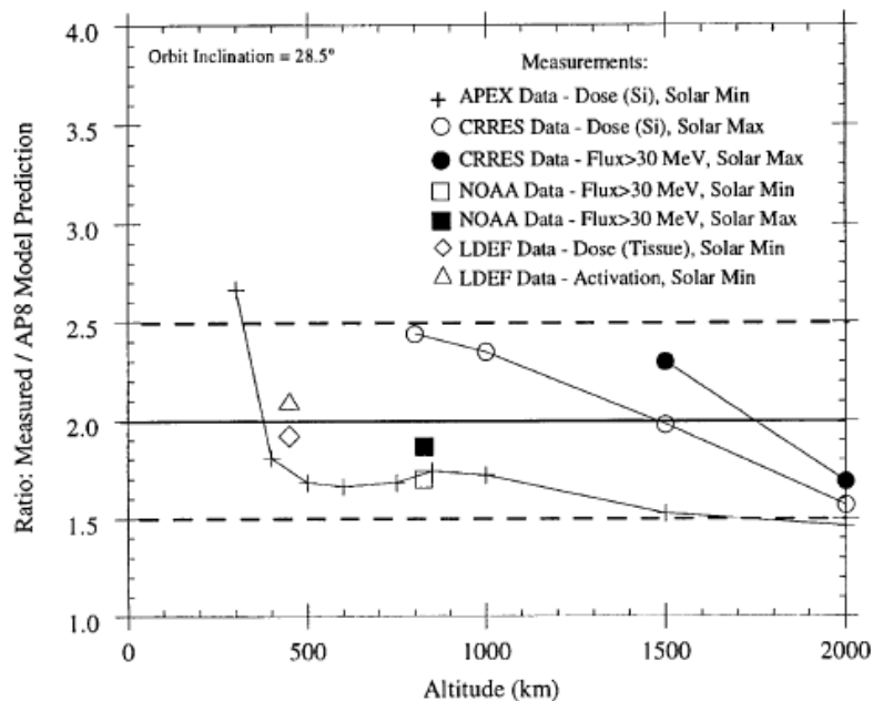
Figure 3: Comparison of flight data with predictions using AP8 trapped proton model for circular orbits with 28.5^\circ inclination [RD-16].
