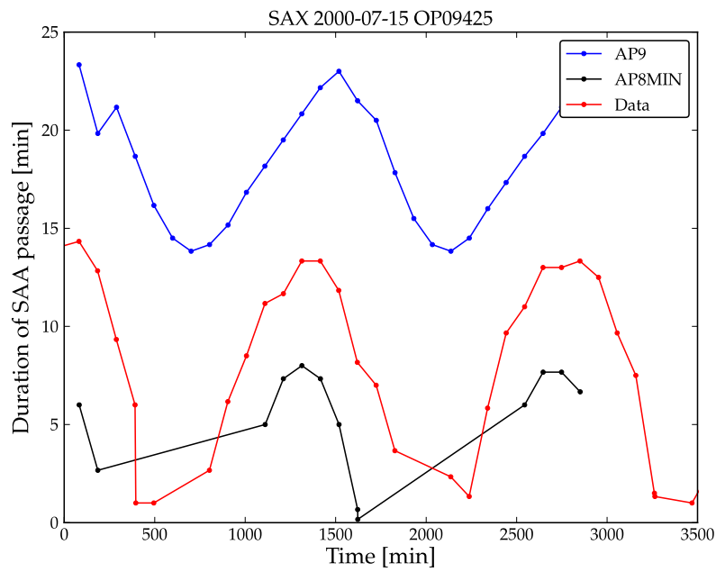
Figure 25: Duration of the passage through the SAA from AP8MIN (black line), AP9 (blue line) and PM data (red line) for a mean altitude of 562 km (OP 9425).
