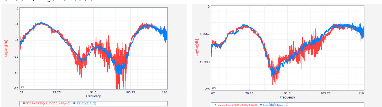
Figure 59 Left panel: Return Loss of the combination S217+S220 (red, reduced bias) vs S217 (blue, nominal bias); Right panel Return Loss of the combination S220+S217 (red, reduced bias) vs S220 (blue, nominal bias).
