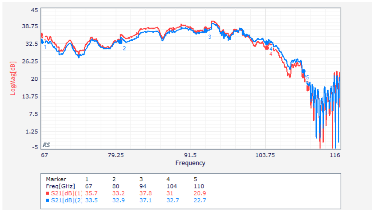
Figure 50 VNA input level @-40 dBm: Insertion gain variation when S220 Id bias is lowered from 20 mA (nominal) to 15 mA (reduced). OK
