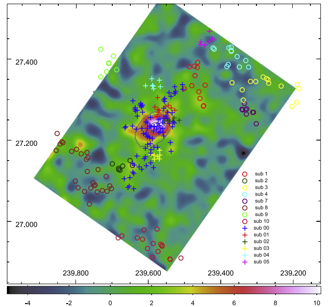
Figure 12. Weak-lensing mass map superimposed with the substructures identified with the \sigma -plateau algorithm. The color code shows the weak-lensing S/N, namely the surface mass density in units of the 1\sigma reconstruction error.
