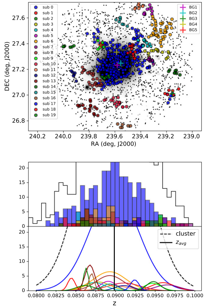
Figure 6. The upper panel shows the distribution on the sky of the A2142 substructures identified with the second threshold. The white contours and grayscale of the background image show the X-ray surface brightness from the combined X-ray observations of XMM (Tchernin et al. 2016). The middle and bottom panels show the velocity histograms of the substructures and their best Gaussian fits. The black vertical line shows the position of the mean redshift z_{\text{avg}} = 0.08982 \pm 0.00010 as a reference.
