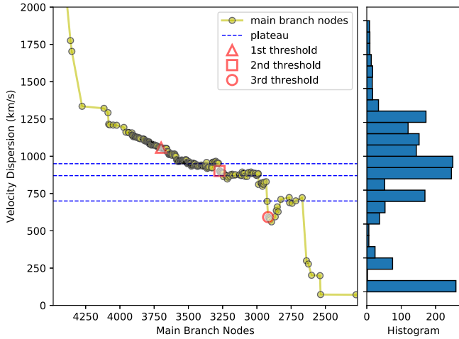
Figure 4. Velocity dispersion of the leaves of each node along the main branch of the binary tree of A2142. The histogram on the right panel shows the node numbers in different velocity dispersion bins. The blue dashed lines indicate the \sigma plateaus. The red symbols are the selected thresholds.
