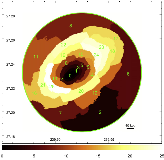
Figure 9. Region map produced on the basis of the surface brightness contours. The color bar denotes the serial number of the regions and has no physical meaning.
