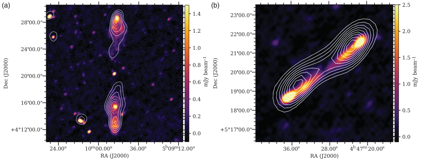
Figure 3. Images from ASKAP-B+0.5 at 887 MHz of two radio galaxies in the field mentioned by VA18. The white contours are MWA-2 at 154 MHz, starting at 3\sigma and increasing in increments of +2\sigma . (a) RA 5^{\text{h}}9^{\text{m}}50^{\text{s}} Dec 4^{\circ}20'19'' and (b) RA 4^{\text{h}}47^{\text{m}}23.9^{\text{s}} Dec 5^{\circ}18'50'' .
