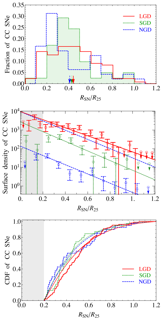
Figure 2. Upper panel: distributions of deprojected and normalized galactocentric radii ( \bar{r} = R_{\text{SN}}/R_{25} ) of CC SNe in LGD (red solid), SGD (green dotted), and NGD (blue dashed) host galaxies. The mean values of the distributions are shown by arrows. Middle panel: surface density distributions (with arbitrary normalization) of CC SNe in the mentioned hosts. For better visualization, thanks to more data points, the bin size of distribution in LGD galaxies is 0.05, in units of R_{25} , while for the other subsamples the bin size is 0.1. The error bars assume a Poisson distribution. The upper limits of surface density (with +1 SN if none is found) are represented by down arrows. The fitted exponential surface density profiles are estimated for the inner-truncated discs (outside the shaded area). For better visibility, the distributions and profiles are shifted vertically and then sorted by increasing the mean \bar{r} as one moves upwards, and also slightly shifted horizontally. To visually compare the distribution of CC SNe in LGD hosts with the fitted profile in NGD galaxies, the latter is also positioned with the central surface density matched with that in LGD hosts. Bottom panel: inner-truncated cumulative distributions of SN radii and their best-fitting exponential CDFs.
