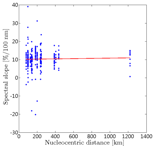
Figure 12. Spectral slopes between [535–882] nm versus the nucleocentric distance. Each blue point represents the spectral slope obtained from the 3-point spectra fit.
