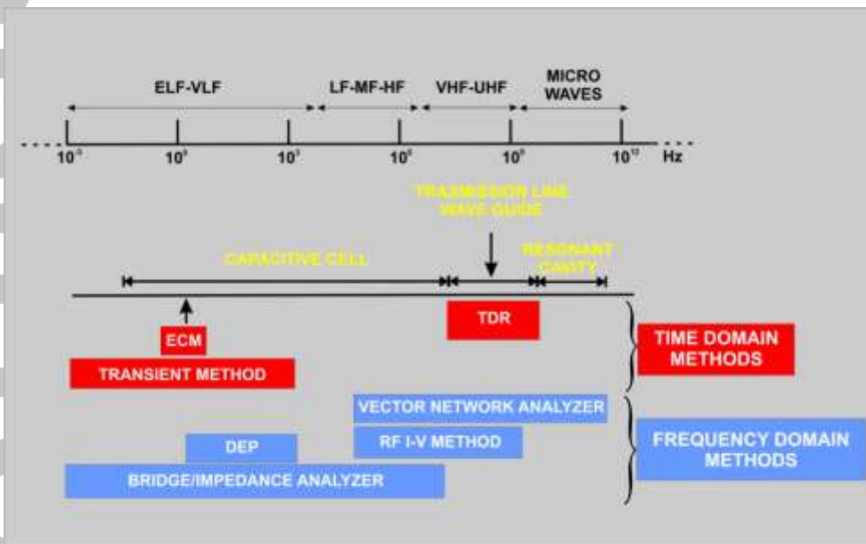
Figure a Dielectric measurement methods in the electromagnetic spectrum (not in scale)
