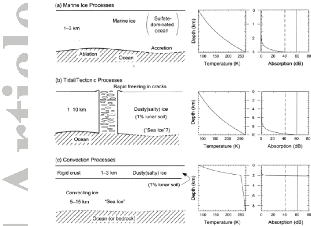
Figure 18 Europa icy crust models proposed by Moore [2000] (left) and relevant radar signal absorption vs. depth (right) [taken from Blankenship et al. , 2009]. a) Conductive ice shell similar to terrestrial marine ice; b) icy crust subjected to tectonic process with extrusions of molten material; c) convective ice shell below a thin rigid stagnant lid. Dashed and solid lines in right panels represent the expected signal to noise ratio for the jovian and anti-jovian sides.
