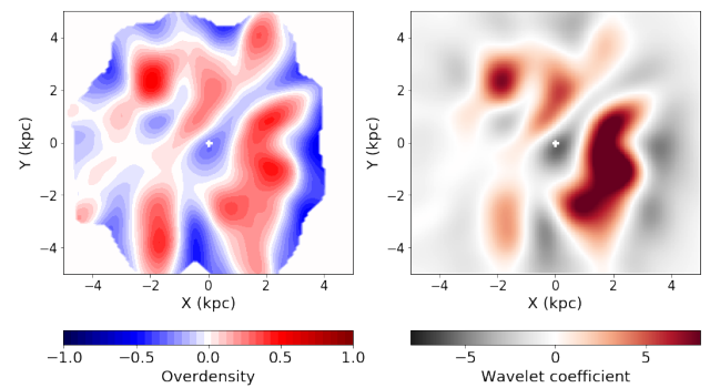
Fig. B.2. Same as Figure 1B (left panel) and C (right panel), but using a larger scale length h = 0.8 kpc, which corresponds to scale=4 of the wavelet transform.
