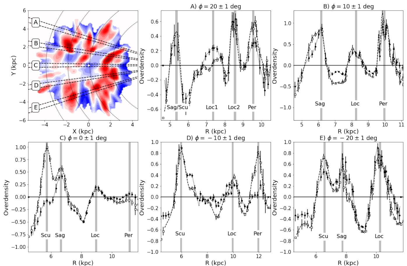
Fig. 2. Top left panel: Same as Figure 1B, but with some geometric references superimposed. Dotted lines from left to right show the points with constant Galactocentric radius R=12,10,8,6 kpc, respectively. Dashed lines show the five selected slices (A,B,C,D,E), which are separated by 10 deg in Galactic azimuth \phi and of 2 deg in width. Panels A to E: The profile of the measured overdensity as a function of R for the UMS P18 sample (black dots) and the Z21 sample (white squares). Error bars show bootstrap uncertainties, calculated as explained in Appendix B.3. For computational reasons, black dots/white squares and relative errorbars were calculated for each slice and then connected using splines, as shown by the dotted (dashed) lines, to give a visual impression of how the overdensity varies at different radii. Each peak of the measured overdensity has been identified with a spiral arm in the Milky Way, as indicated by the vertical grey lines and the corresponding labels. The identification of each peak is not due to an assumed specific model, but is simply based on the geometric appearance of the top left panel (see text).
