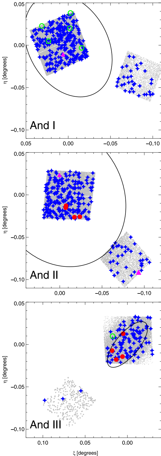
Figure 3. Spatial distribution of the variable stars found in the observed ACS +WFC3 fields for And I, II, and III. Non-variable stars are represented by gray dots. Variables are shown with the same symbol and color code as in Figure 1. The black ellipses represent the half-light radius ( r_h ) for each galaxy (column 6 in Table 1).
