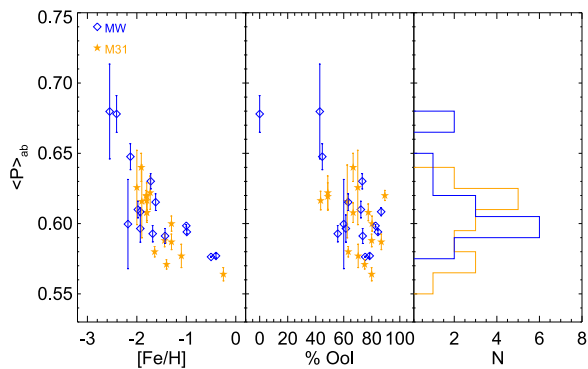
Figure 8. Left and middle panel: mean period of the RRab stars of the sample of MW (blue) and M31 (orange) satellites vs. the mean metallicity and the percentage of Oo-I type stars in the system. There is no obvious difference between the two subgroups. Right panel: mean period distribution of the sample of MW (blue histogram) and M31 dwarf galaxies (orange histogram). The peaks of the two distribution are very close to each other.
