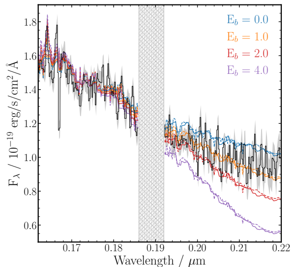
Figure 12. Investigating evidence for excess attenuation at 2175Å from a composite of 122 VANDELS spectra at 3.0 \leq z \leq 3.5 ( \langle z \rangle = 3.288 ). The grey spectrum is the composite VANDELS spectrum with the grey shaded region representing the \pm 1\sigma error. The hatched region around \lambda \sim 0.19\mu\text{m} masks the \text{C III]}\lambda 1909 emission line. The solid and dashed coloured curves show, respectively, the FiBY-BPASSv2-300bin and S99-v00-z008 templates reddened using the Noll et al. (2009) attenuation curve assuming four values of the 2175Å bump strength ( E_b ; see text for details). For each value of E_b the templates have been attenuated with A_V = 0.8 assuming the Calzetti A_V - M_* relation at the median mass of the galaxies contributing to the stack ( \log(M_*/M_\odot) = 9.71 ; see Fig. 9).
