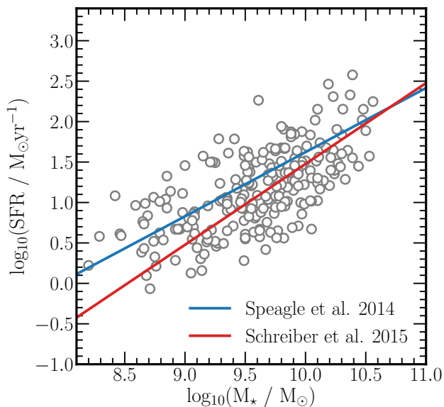
Figure 1. The position of our VANDELS sample in the M_* -SFR plane. Masses and star-formation rates were derived using the SED fitting code LEPAHRE (see text for details). For comparison, the blue and red lines show two independent determinations of the main sequence of star formation at z = 3.5 from Speagle et al. (2014) and Schreiber et al. (2015) respectively. It can be seen that the galaxies in our sample are consistent with being typical star-forming galaxies at z = 3.5 .
