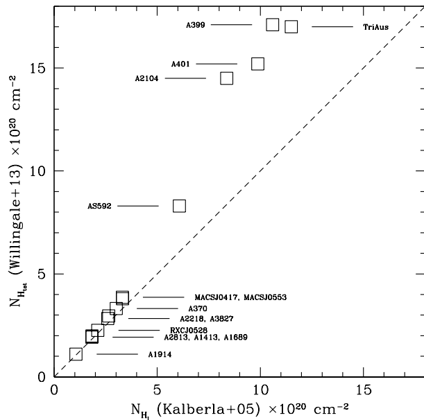
Figure 1. Comparison between the H_I density column from Kalberla et al. (2005) and the total ( H_I+H_2 ) density column from Willingale et al. (2013). The dashed line indicates the linear correlation as a reference.
