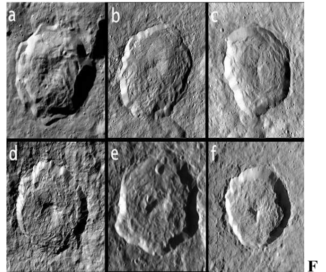
fig. 26. Comparison of immature complex craters on Ceres (a–c) and on icy Saturnian satellites (d–f). Ceres craters are between 20 and 40 km across. Crater (d) is Telemachus (D = 95 km) and (f) is Sagaris (D = 45 km), also highlighted in Fig. 10. Craters shown at similar apparent diameter (and at different scales) to facilitate structural comparison.
