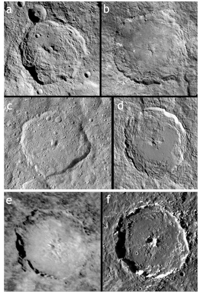
Fig. 19. Central pit craters on Ceres (top two rows) as compared to Ganymede and Callisto (bottom row). Ceres (top rows): (a) Toharu, 82 km, with summit pit; (b) Dantu, 119 km, with floor pit; (c) Nawish, 77 km; (d) Occator, 92 km (shown as shaded relief of topography due to high contrast of central pit). Ganymede and Callisto (bottom row): (e) central pit crater on Ganymede, 70 km, with floor pit; (f) central pit crater on Callisto, 65 km, with floor pit and partial rim massif to the east, similar to Occator. See also central pit crater Gaue (Ceres) in Fig. 16. Images are not to same scale.
