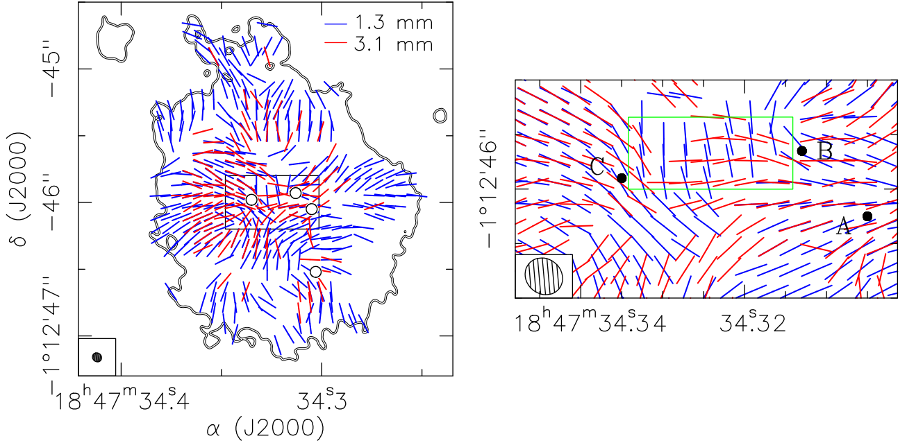
Fig. 5. Comparison of magnetic field orientations at 1.3 mm and 3.1 mm. Left: Magnetic field segments at 1.3 mm (blue) and 3.1 mm (red). Segments shown every ten pixels. Contours show the 5 \sigma -level dust continuum emission at 1.3 mm. The synthesized beam is shown in the lower left corner. The black rectangle indicates the zoomed region shown in the right panel. Right: Close-up of the central region toward sources A, B, and C. Segments are shown every five pixels. The green rectangle shows the region where the polarization segments at 1.3 mm and 3.1 mm are almost perpendicular.
