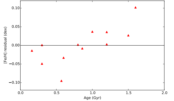
Fig. 5. Residuals in [Fe/H] from the linear gradient as a function of cluster age.
