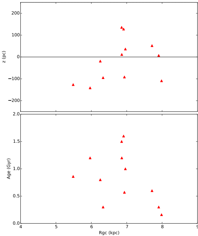
Fig. 1. Top panel: locations of the GES open clusters (red triangles) relative to the Galactic plane ( z = 0 , solid line), as a function of their Galactocentric radii. All clusters lie within 150 pc of the mid-plane, and thus are members of the thin disk. Bottom panel: cluster ages (in Gyr) plotted as a function of R_{GC} .
