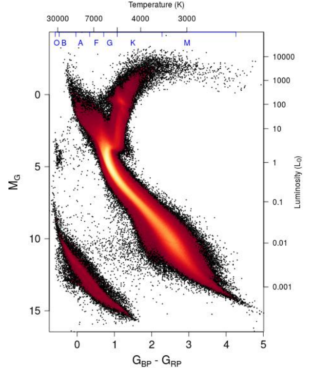
Fig. 5. Gaia HRD of sources with low extinction ( E(B-V) < 0.015 mag) satisfying the filters described in Sect. 2.1 (4276690 stars). The colour scale represents the square root of the density of stars. Approximate temperature and luminosity equivalents for main-sequence stars are provided at the top and right axis, respectively, to guide the eye.
