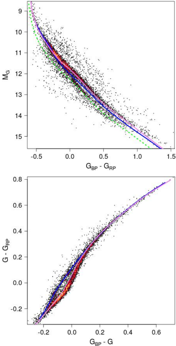
Fig. 14. Gaia HRD of white dwarfs with \sigma_w/\varpi < 5\% and \sigma_{G_{BP}} < 0.01 and \sigma_{G_{RP}} < 0.01 (5 781 stars) overlaid with white dwarf evolutionary models. Magenta: 0.6 M_{\odot} pure H; green dashed: 0.8 M_{\odot} pure H; and blue: 0.6 M_{\odot} pure He. Panel a : HRD. Panel b : colour–colour diagram.
