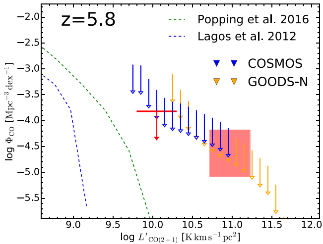
Figure 4. VLA COLDz CO( J = 2 \rightarrow 1 ) luminosity function at \langle z \rangle = 5.68 and 5.86 in the COSMOS (blue and red arrows) and GOODS-North (orange arrows and red boxes) fields, respectively. The blue and orange arrows show upper limits under the unlikely assumption that any candidates not independently be confirmed to be CO( J = 1 \rightarrow 0 ) emission would correspond to CO( J = 2 \rightarrow 1 ) emission, for the same binning in L'_{\text{CO}} as in Figure 2. Red arrows and boxes consider only independently confirmed CO( J = 2 \rightarrow 1 ) candidates. The dashed lines show the model predictions.
